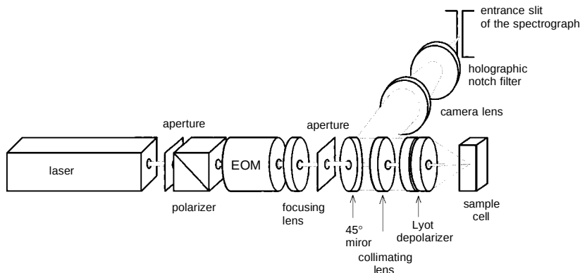
FIG. 1 Optical layout of the ROA spectrometer
